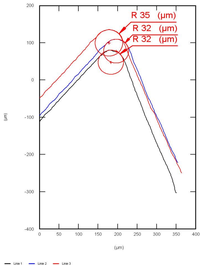
Fig.: Cutting edge after processing
